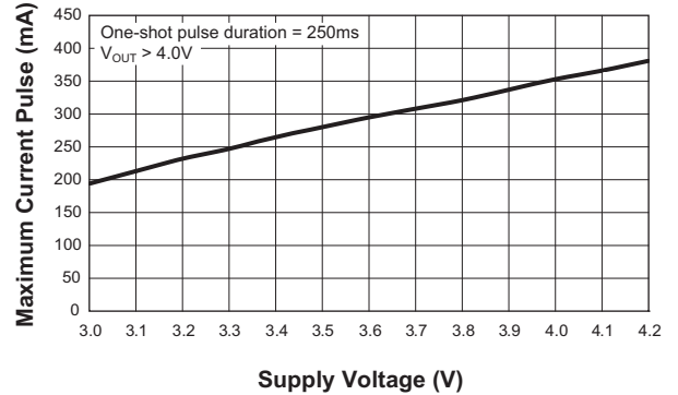
Maximum Current Pulse vs. Supply Voltage
