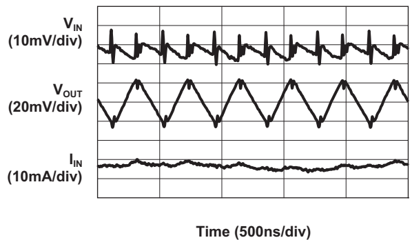
Output Ripple Voltage vs. Time
