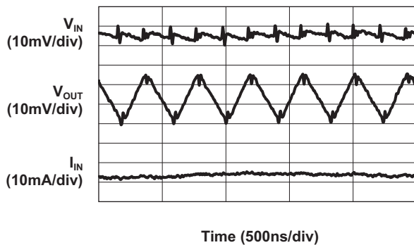
Output Ripple Voltage vs. Time
