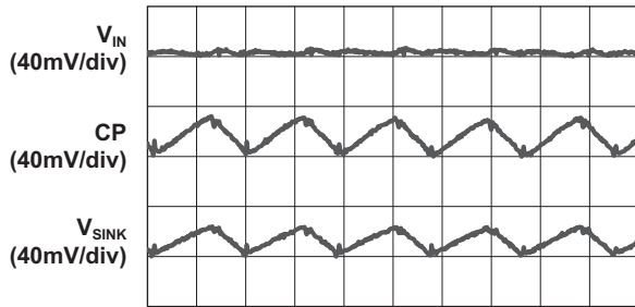
Load Characteristics ( V_{IN} = 3.7V ; 1.5X Mode; 15mA Load)
